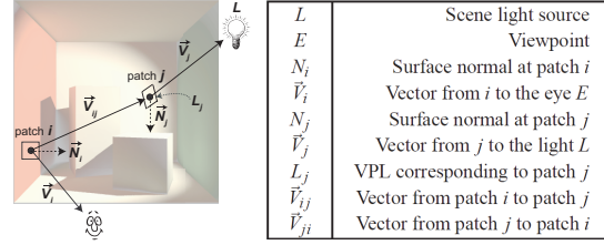
Figure 4: Notation used for image-space radiosity.
