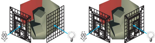
Figure 6: (Left) Multiresolution splatting has temporal coherence issues when light samples jump suddenly from one surface to another. This is due to poor light-space patch selection. (Right) Using multiresolution VPLs lessens this problem, as VPLs near boundaries split into multiple, less important patches.
